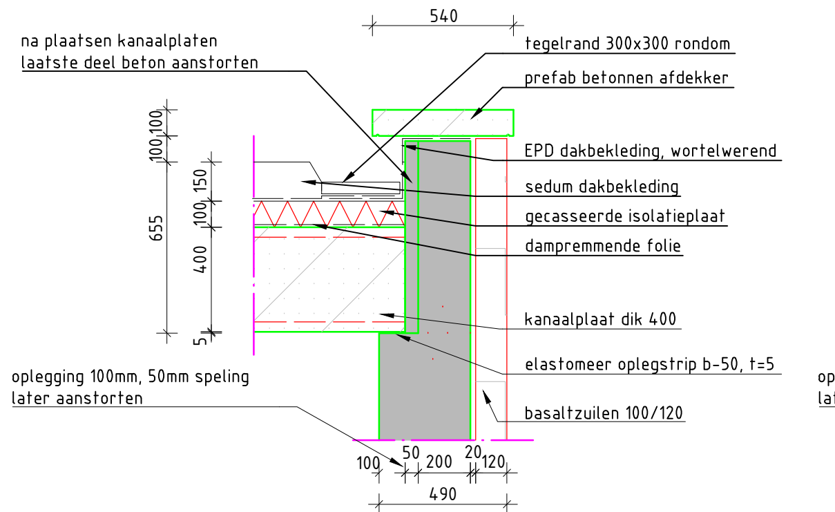
DETAIL 1: OPLEGGING schaal 120
