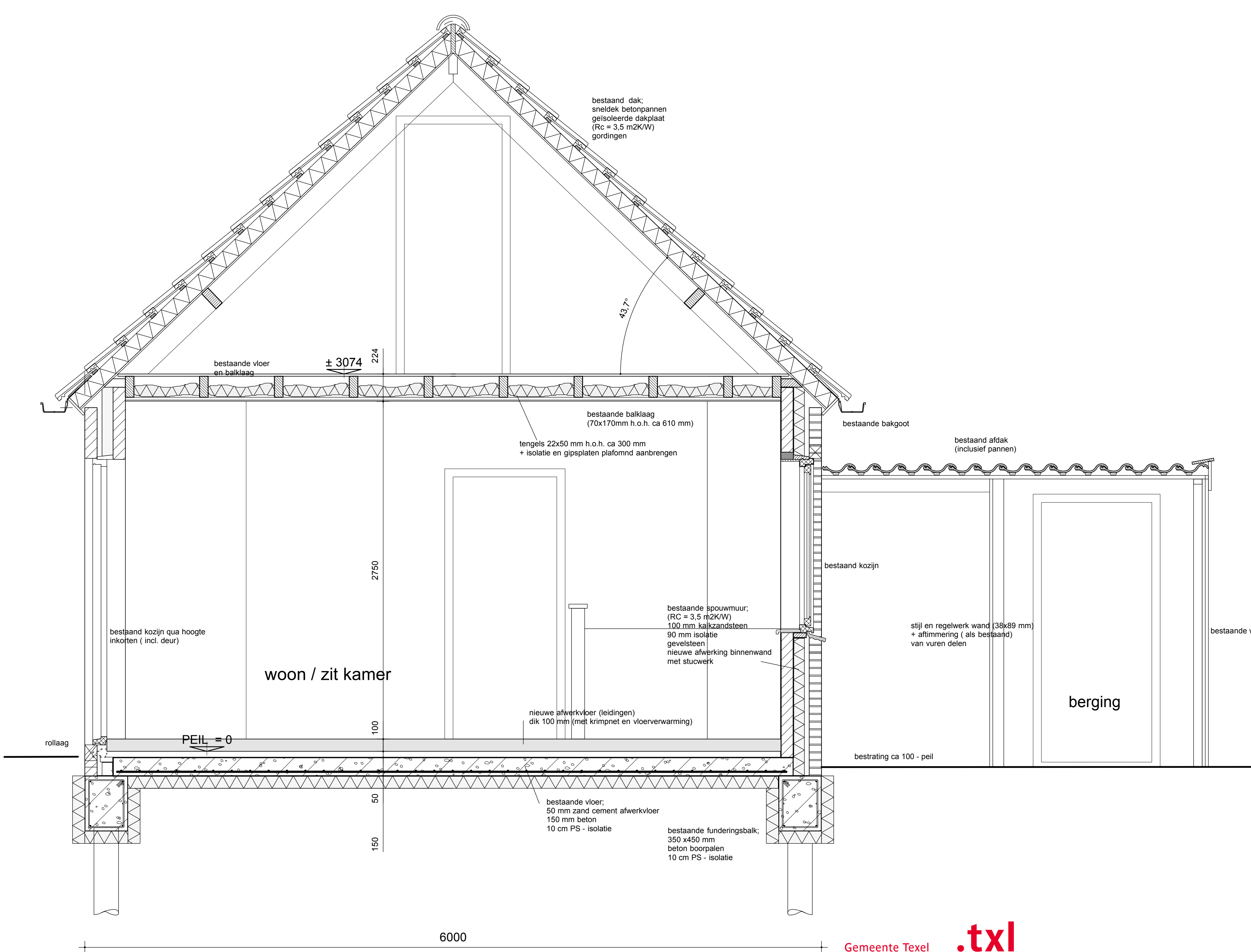
principe detail - dwarsdoorsnede
